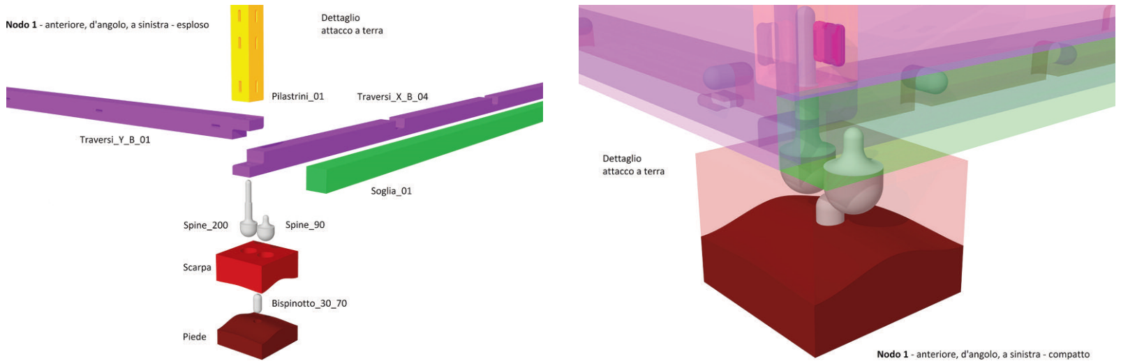
Figg. 5, 6 - Left: Exploded perspective view Node 1. Right: Compact perspective view Node 1, with transparent surfaces.
